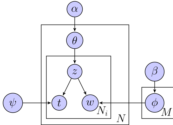
Figure 7.2: Bayesian network describing how TOT generates a corpus of data; see Algorithm 7.4.
